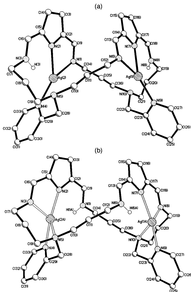
Fig. 4 Perspective views of the (a) the major component and (b) the minor component of the cation [\text{Ag}_2(\text{H}_2\text{L}^4)]^{2+} .
